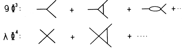
FIG. 2. Radiative corrections to \Phi^3 and \Phi^4 interactions.
