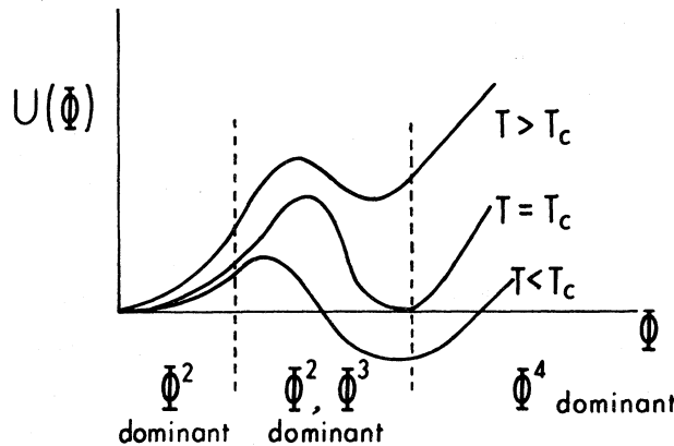
FIG. 1. The potential U(\Phi) of Eq. (10) at different temperatures.
