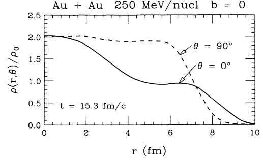
FIG. 2. Baryon density along (solid line) and perpendicular (dashed line) to the beam axis at t = 15.3 fm/c, in the b = 0 Au + Au collision at beam energy of 250 MeV/nucleon.
