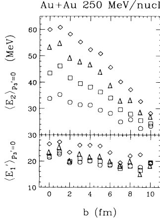
FIG. 11. Mean out-of-plane \langle E_2 \rangle and in-plane \langle E_1 \rangle kinetic-energy components of protons (circles), deuterons (squares), tritons (triangles), and helions (diamonds), at p_3 \approx 0 . The directions 1' and 3' are, respectively, along the minor and major axis of the sphericity tensor (3.2) in the reaction plane, while the direction 2 is out of the reaction plane.
