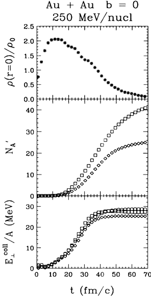
FIG. 4. Time dependence of different quantities in the b=0 Au+Au reaction at 250 MeV/nucleon. Top panel displays the baryon density at r=0 . Squares in the center panel indicate the number of deuterons, and diamonds the number of A=3 clusters, which survive intact till the end of the reaction. Diamonds, squares, and circles, in the bottom panel, indicate the collective energy per nucleon (3.1) of A=3 clusters, deuterons, and nucleons, respectively.
