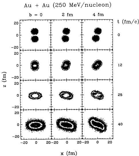
FIG. 1. Contour plots of the particle density integrated over the normal to the reaction plane in Au+Au collisions at 250 MeV/nucleon.
