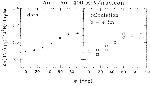
FIG. 6. Azimuthal distribution about the beam axis at the c.m. longitudinal momentum p_{\parallel} \approx 0 , in the semicentral Au+Au collisions at 400 MeV/nucleon. Left panel shows the distribution of all particles, in the third of five multiplicity bins, as determined in the experiment of Ref. [5]. Squares and circles in the right panel indicate, respectively, the calculated deuteron and proton distributions, at b = 4 fm.
