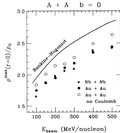
FIG. 3. Maximum densities reached in the b = 0 collisions of heavy nuclei, as a function of the bombarding energy per nucleon. The solid line shows the densities obtained by solving the Rankine-Hugoniot relations for a shock wave [18].
