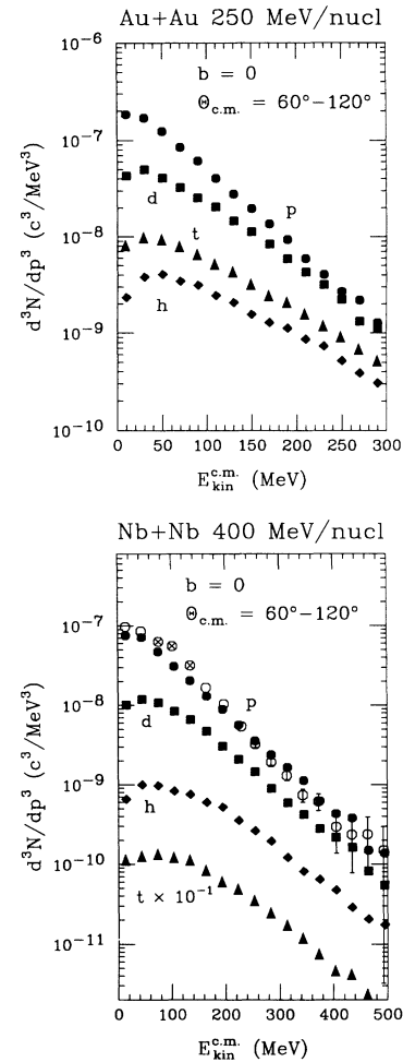
FIG. 10. Spectra of protons (filled circles), deuterons (squares), tritons (triangles), and helions (diamonds) from the b=0 Au+Au reaction at 250 MeV/nucleon, and from the b=0 Nb+Nb reaction at 400 MeV/nucleon, in the range of the c.m. polar angle \theta between 60^\circ and 120^\circ . Open circles for the Nb+Nb reaction represent the proton spectrum at 90^\circ , in arbitrary units, measured in Ref. [24] in events with charged-particle multiplicity between 50 and 60. Crossed circles indicate region where proton spectra were contaminated by misidentified deuterons and tritons.
