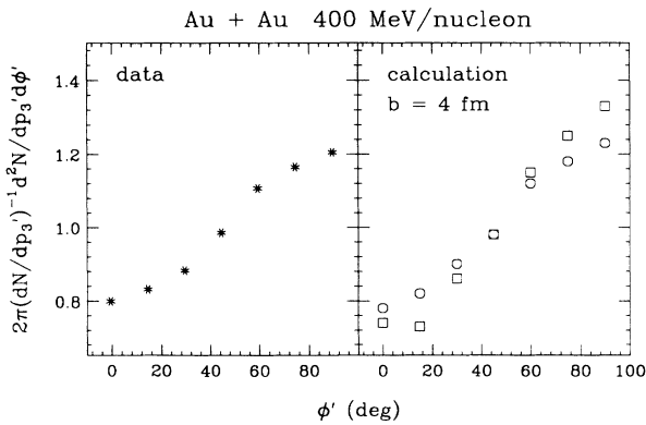
FIG. 7. Azimuthal distribution about the major axis of the sphericity tensor (3.2), at the momentum component along the axis p_y \approx 0 , in the semicentral Au+Au collisions at 400 MeV/nucleon. Left panel shows the distribution of all particles, in the third of five multiplicity bins, as determined in the experiment of Ref. [5]. Squares and circles in the right panel indicate, respectively, the calculated deuteron and proton distributions, at b = 4 fm.
