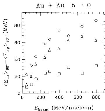
FIG. 12. Differences between mean kinetic energies of composite particles and proton energies at 90^\circ in the b=0 Au+Au collisions, as a function of beam energy. The deuteron-proton differences are represented by squares; triton-proton differences by triangles; and helion-proton differences by diamonds. The scatter of points reflects statistical errors of the calculations.
