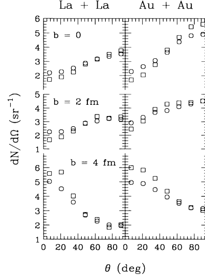
FIG. 5. Number of protons (circles) and deuterons (squares) emitted per unit spherical angle, as a function of the c.m. polar angle \theta , in the La+La collisions at 246 MeV/nucleon, and in the Au+Au collisions at 250 MeV/nucleon, at different impact parameters.
