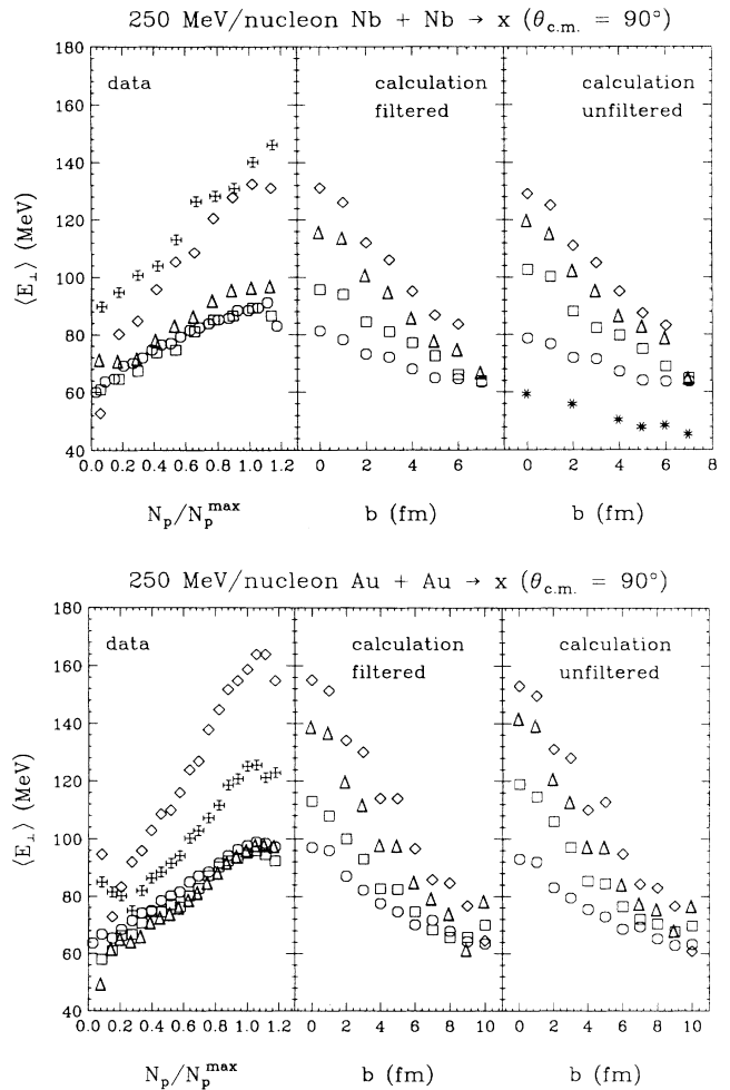
FIG. 8. Mean kinetic energies of protons (circles), deuterons (squares), tritons (triangles), and helions (diamonds) at c.m. polar angle of 90^\circ , in the Nb+Nb and Au+Au collisions at 250 MeV/nucleon. Left panels display the mean energies determined in the experiment of Ref. [8], as a function of normalized multiplicity. Center and right panels show the results of our calculations as a function of impact parameter in the direct form, and with the final state subjected to a filtering procedure (Ref. [22]), respectively. Proton energies in the Nb+Nb collisions, obtained with the composite production switched off, are indicated by stars.
