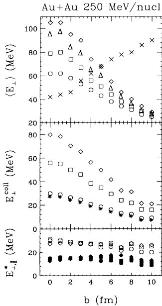
FIG. 9. Different energies calculated in the Au+Au collisions at 250 MeV/nucleon, as a function of the impact parameter. The top panel shows the final transverse energies averaged over all angles of protons (circles), deuterons (squares), tritons (triangles), and helions (diamonds). Crosses in the top panel indicate twice the mean longitudinal proton energy. The center panel shows collective transverse energy (3.1) of nucleons (circles), deuterons (squares), and A=3 clusters (diamonds). Stars in the center panel indicate mean transverse energy per nucleon of all particles. Bottom panel shows the longitudinal (filled symbols) and transverse (open symbols) excitation energies at freeze out, Eq. (3.10), of nucleons (circles), deuterons (squares), and A=3 clusters (diamonds).
