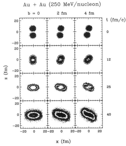
FIG. 1. Contour plots of the particle density integrated over the normal to the reaction plane in Au+Au collisions at 250 MeV/nucleon.
