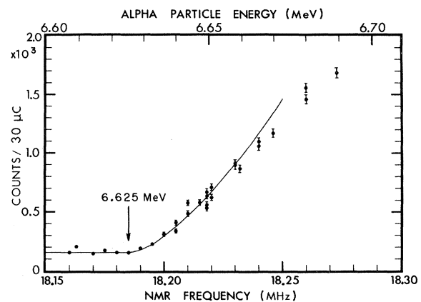
FIG. 3. The neutron yield at 0^\circ vs E_\alpha from the ^6\text{Li}(\alpha, n)^9\text{B} neutron near threshold. The calculated curve assumes the expected s -wave threshold for a thick target and a constant background, and fits the data below 18 240 kHz for a threshold at \nu = 18 185 \pm 2 kHz. The magnetic-analyzer constant derived from this measurement is in excellent agreement ( <150 ppm) with three earlier calibrations extending over 5 yr.
