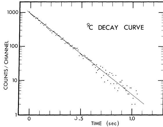
FIG. 4. Delayed-proton counts per 10-msec time bin in a cyclic multiscaler. The curve is a least-squares fit of the form N e^{-t/\tau} + C , with \tau = 126.5 \pm 1.7 msec and C = 0.1 \pm 1.7 ; \chi^2 = 1.2 per degree of freedom.
