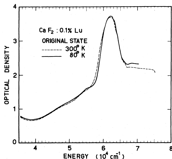
FIG. 6. Ultraviolet absorption spectra of PC in \text{CaF}_2:0.1\%\text{Lu} .
