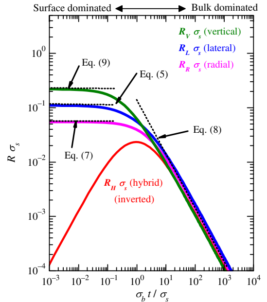
FIG. 9. Example of numerical results for a two-terminal double-sided Corbino disk. Numerical result of R_L \sigma_s (the blue line), R_R \sigma_s (the magenta line), R_V \sigma_s (the green line), and R_{\text{inv}} \sigma_s (the red line) vs x (= \sigma_b t / \sigma_s) when the thickness is t = 100 \mu\text{m} . The dotted lines indicate the asymptotic values from the equations.
