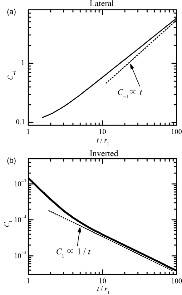
FIG. 7. The transport coefficients for the single-sided four-terminal Corbino disk geometry as a function of sample thickness. (a) C_{-1} of the lateral resistance R_L in the bulk-dominated regime ( \sigma_b t \gg \sigma_s ). (b) C_1 of the inverted resistance R_{\text{inv}} in the surface-dominated regime ( \sigma_s \gg \sigma_b t ). The thickness is dividing by r_1 ( = 100 \mu\text{m} ). The dotted lines indicate the transport coefficients when they are independent of thickness.
