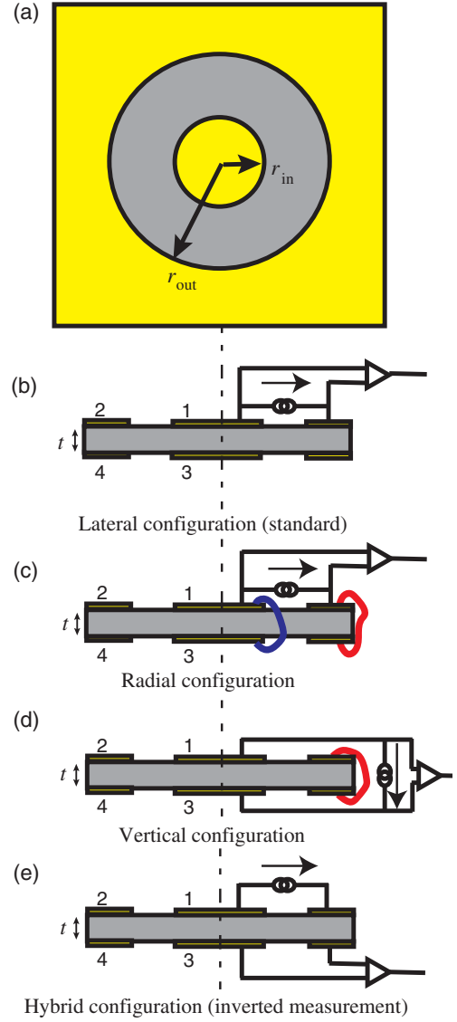
FIG. 8. Double-sided two-terminal Corbino disk. The sample is shown in gray and the highly conductive contacts are shown in yellow. (a) Top and bottom surface view. (b) Side view and the lateral resistance configuration. (c) Side view and the radial resistance configuration. The blue and red lines are jumper wires. (d) Side view and the vertical resistance configuration. (e) Side view and the hybrid resistance configuration. The hybrid measurement is an inverted resistance measurement in the surface-dominated regime ( \sigma_s \gg \sigma_b t ). We choose the Corbino dimensions as r_1 = 150 \mu\text{m} and r_2 = 300 \mu\text{m} .
