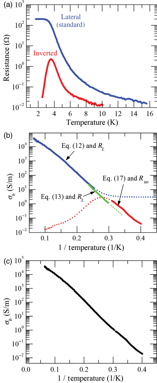
FIG. 13. Experimental results and bulk conductivity analysis on a single-sided four-terminal Corbino disk on a \text{SmB}_6 sample with a thickness t = 300 \mu\text{m} . (a) Resistance vs temperature of the lateral and inverted measurements. (b) The bulk conductivity converted from the measured resistance. The dotted lines indicate the bulk conductivity conversion applied beyond the appropriate regime. (c) The result of the extracted bulk conductivity after an adjustment of mismatch.
