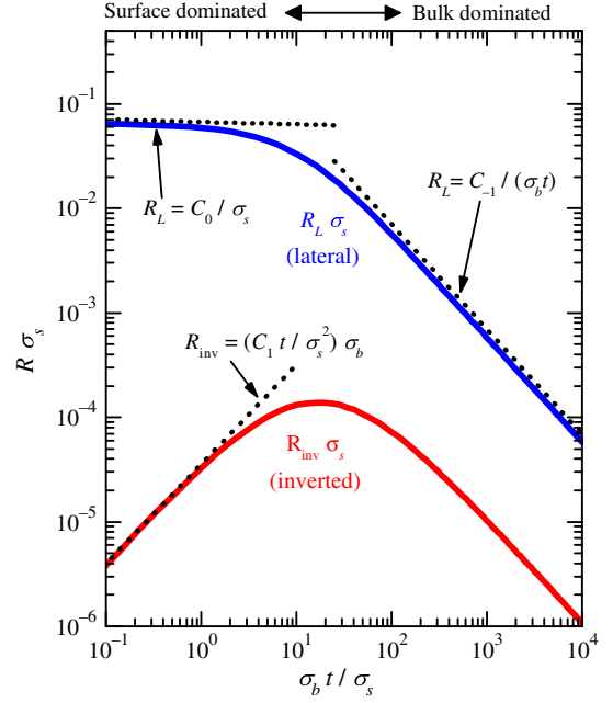
FIG. 6. Example of numerical results of a single-sided Corbino disk. R_L\sigma_s (the blue line) and R_{\text{inv}}\sigma_s (the red line) as a function of x (= \sigma_b t / \sigma_s) when t = 1000 \mu\text{m} . The dotted lines represent the asymptotic values from the first-order term from Eqs. (2)–(4).
