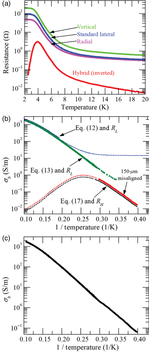
FIG. 14. Experimental results and bulk conductivity analysis of the double-sided two-terminal Corbino disk on a \text{SmB}_6 sample with a thickness t = 210 \mu\text{m} . (a) Resistance vs temperature of the lateral, vertical, radial, and hybrid measurements (inverted measurement). (b) The bulk conductivity converted from the measured resistance shown in (a). The dotted lines indicate the bulk conductivity conversion applied beyond the appropriate regime. (c) The result of the bulk conductivity after an adjustment of mismatch.
