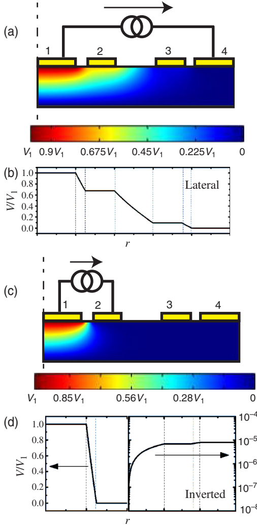
FIG. 5. The potential distributions of the single-sided four-terminal Corbino disk. The bulk and the surface are calculated in the surface-dominated transport regime ( \sigma_s \gg \sigma_b t ); t = 100 \mu\text{m} , \sigma_b = 0.00131/(\Omega \text{ m}) , and \sigma_s = 0.0051/\Omega . The equipotential values are normalized by the potential at the current source ( V_1 ). (a) Potential distribution in the bulk when the current is connected to the lateral configuration. (b) Potential distribution on the surface as a function of radial position when the current is connected to the lateral configuration. (c) Potential distribution in the bulk when the current is connected to the inverted configuration. (d) Potential distribution on the surface as a function of radial position when the current is connected to the inverted configuration. The surface region in r < r_{\text{in}} is plotted in a linear scale, and r > r_{\text{in}} is plotted in a logarithmic scale.
