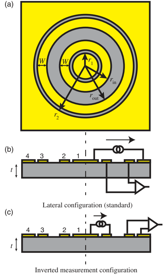
FIG. 4. Four-terminal single-sided Corbino disk. The sample is shown in gray and the highly conductive contacts are shown in yellow. (a) Top view. (b) Side view and resistance configuration of the lateral configuration. (c) Side view and the resistance configuration of the inverted measurement configuration. We choose the dimensions: r_1 = 100 \mu\text{m} , r_2 = 800 \mu\text{m} , r_{\text{in}} = 200 \mu\text{m} , r_{\text{out}} = 300 \mu\text{m} , and W = 75 \mu\text{m} .
