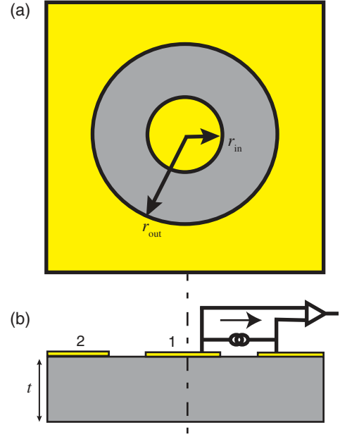
FIG. 2. A standard two-terminal Corbino disk on a sample. (a) (Top view) The sample is shown in gray and the highly conductive contacts are shown in yellow. (b) (Side view) The current and voltage amplifier that is needed to perform the resistance measurements is connected to terminals 1 and 2.
