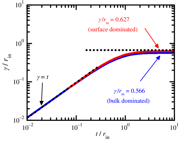
FIG. 3. Effective thickness, \gamma , in the two-channel model vs the real sample thickness, t , for a standard Corbino disk. Both axes are divided by the inner radius ( r_{\text{in}} = 150 \mu\text{m} ). The solid red line is the numerical calculation in the surface-dominated regime when only the top surface contributes. When the thickness is very large, \gamma/r_{\text{in}} asymptotically approaches 0.627. The solid blue line is the numerical calculation in the bulk-dominated regime. At large thickness, \gamma/r_{\text{in}} asymptotically approaches 0.566. The effective thickness approaches the true thickness of the sample when the sample thickness is sufficiently thin ( \gamma = t ).
