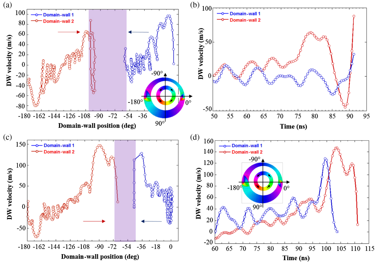
FIG. 4. Micromagnetic simulations of DW dynamics at zero field, comparing the velocity profiles of two different magnetic configurations where the DWs have the same (top) and opposite chiralities (bottom). Panels (a),(b) and (c),(d) show the DW velocities plotted as a function of the azimuthal angle and time for the automotive propagation of two vortex walls with the same and opposite chirality, respectively. The averaged annihilation area where DWs get close enough is indicated in purple. Blue and red arrows indicate the propagation direction of the DWs. Insets in (a) and (d) show the spin structure of the 400-nm ring geometry for both cases with the head-to-head wall on the left and the tail-to-tail wall on the right.
