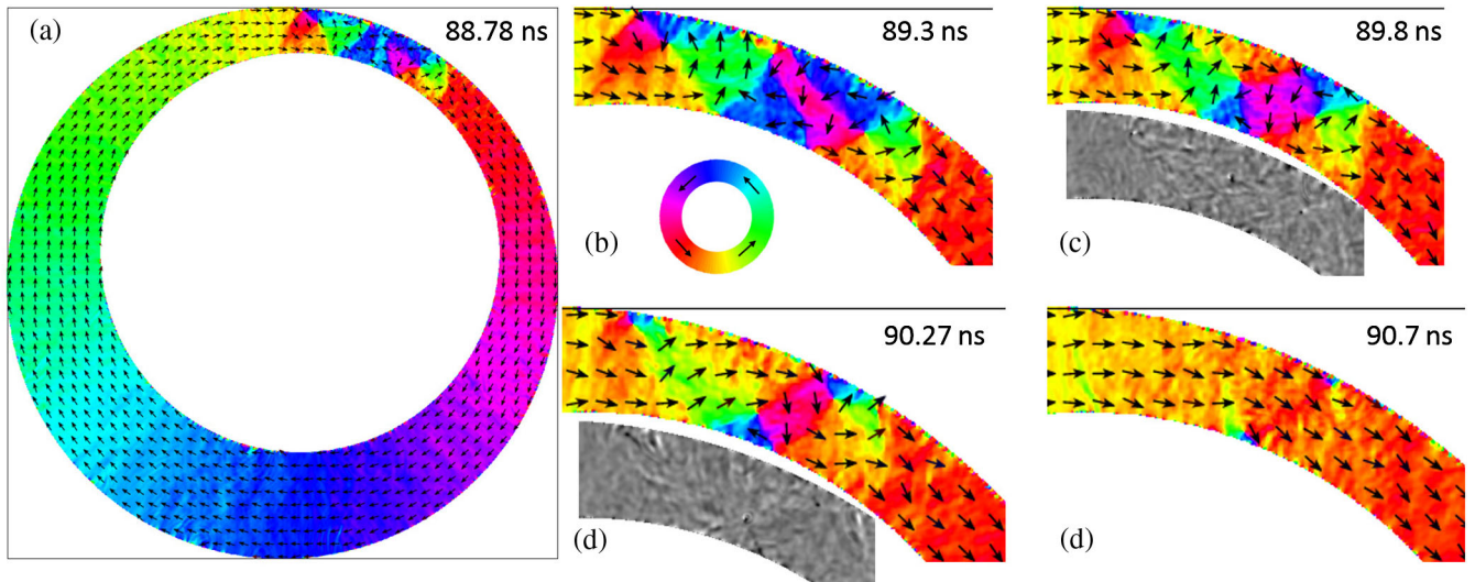
FIG. 5. Micromagnetic simulations for the dynamic vortex DW spin structures during the annihilation process, where DWs have initially the same chiralities and polarities. (a)–(e) Snapshots illustrating the last 2 ns before the full annihilation of the DWs. Insets in (c), (d) show the gray scale of the corresponding snapshots which represent the out-of-plane magnetization component ( M_z ) along the Z direction, where white (black) indicates magnetization pointing up (down). The color code represents the in-plane magnetization direction visualized by the small black arrows.
