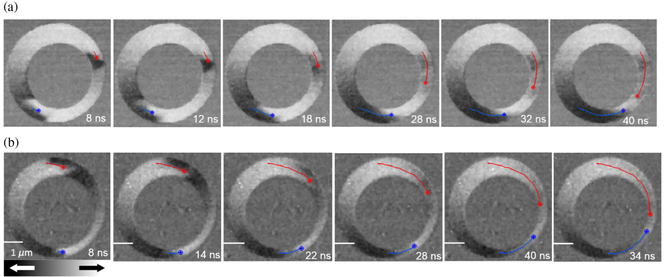
FIG. 3. Time-resolved STXM XMCD snapshots of automotive DWs' motion during the switching process from the onion to the vortex state in the ferromagnetic rings for the case of equal (a) and opposite (b) vortex wall chirality. These snapshots represent part of the XMCD videos used to extract the DW velocities plotted in Fig. 2. Red and blue lines illustrate the averaged trajectory of the vortex wall core of both vortex walls head to head and tail to tail, respectively.
