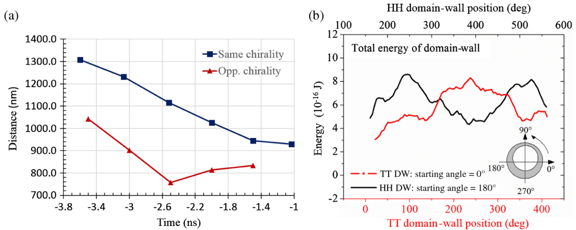
FIG. 7. (a) Calculated distance between vortex cores plotted as a function of time (before the annihilation at t = 0 ns) for both studied cases in Figs. 5 and 6 where the vortex walls have the same and opposite chirality, respectively. (b) Contributions to the DW energy at zero field (exchange + magnetostatic energies) in 500-nm asymmetric rings plotted as a function of DW position. The black and red curves correspond to the head-to-head (HH) and tail-to-tail (TT) vortex wall with a starting or initial angle at 0^\circ and 180^\circ , respectively. The energies are obtained from micromagnetic calculations by propagating the DW along the ring with a field pointing along different directions.
