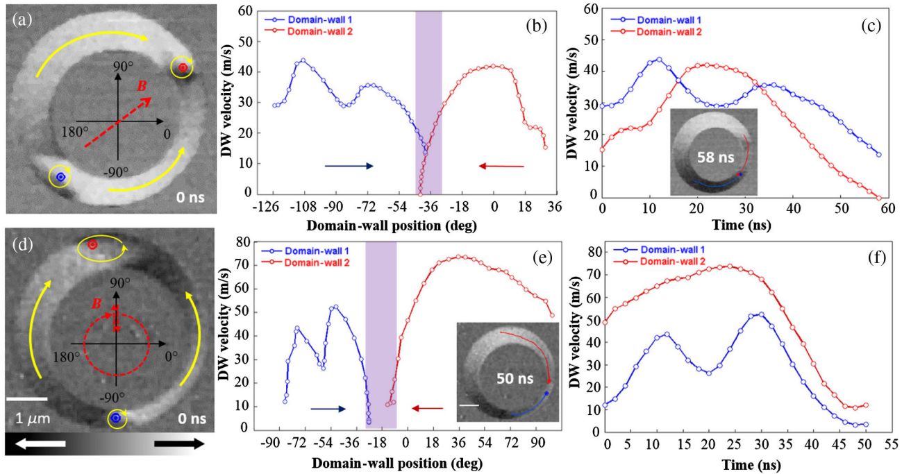
FIG. 2. Automotive DW propagation in an asymmetric ring. (a),(d) Time-resolved XMCD STXM images (at t = 0 ns) showing the relaxed onion state after excitation with a uniform external magnetic field B , with direction indicated by the red arrow either unidirectional (a) or rotational (d), for the case of equal and opposite vortex wall chirality (500 and 400 nm minimum width), respectively. These images visualize the magnetization state just before the start of the automotion process. The vortex core polarity of both vortex walls is indicated in red (head to head) and blue (tail to tail). The yellow arrows indicate the direction of the magnetization. Panels (b),(c) and (e),(f) show the DW velocities (absolute values) plotted as a function of the azimuthal angle and time for the automotive propagation of two vortex walls with the same and opposite chirality, respectively. Blue and red arrows indicate the propagation direction of the DWs. The averaged annihilation area where the DWs get close enough is indicated in purple. Insets in panels (c) and (e) present the time-resolved STXM-XMCD snapshots at t = 58 and 50 ns showing the vortex state (clockwise) after the annihilation process of the DWs for the approach of two vortex walls with same and opposite chirality, respectively. Red and blue lines illustrate the trajectory of the DW vortex core extracted from the time-resolved video. White (black) contrast corresponds to magnetization pointing to the right (left).
