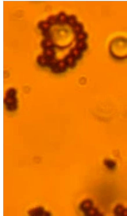
VIDEO 6. Controlled transport of a 3\text{-}\mu\text{m} \text{SiO}_2 particle trapped into a dipolar ring. The ring is transported at a constant speed upon application of a precessing magnetic field with frequency f = 20 Hz and amplitudes H_x - H_e = 0.1 Oe, H_y = 0.7 Oe and H_z = 7.1 Oe. After t = 61 s the field polarity is changed ( H_z = -H_z ) and the translational motion is inverted.
