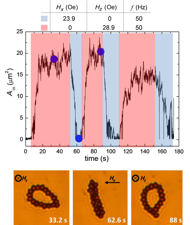
FIG. 3. Time evolution of the area A_{in} of a dipolar ring composed of N = 18 particles and subjected to a 50-Hz oscillating magnetic field applied either perpendicular to the ring ( H_z ) or in the plane of the ring ( H_x ). The solid disks indicate the location of the snapshots displayed at the bottom, which show the ring deformations.
