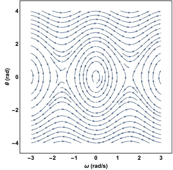
FIG. 5. Phase portrait of the dynamical system given by Eq. (C3) for C_m = 5 .
