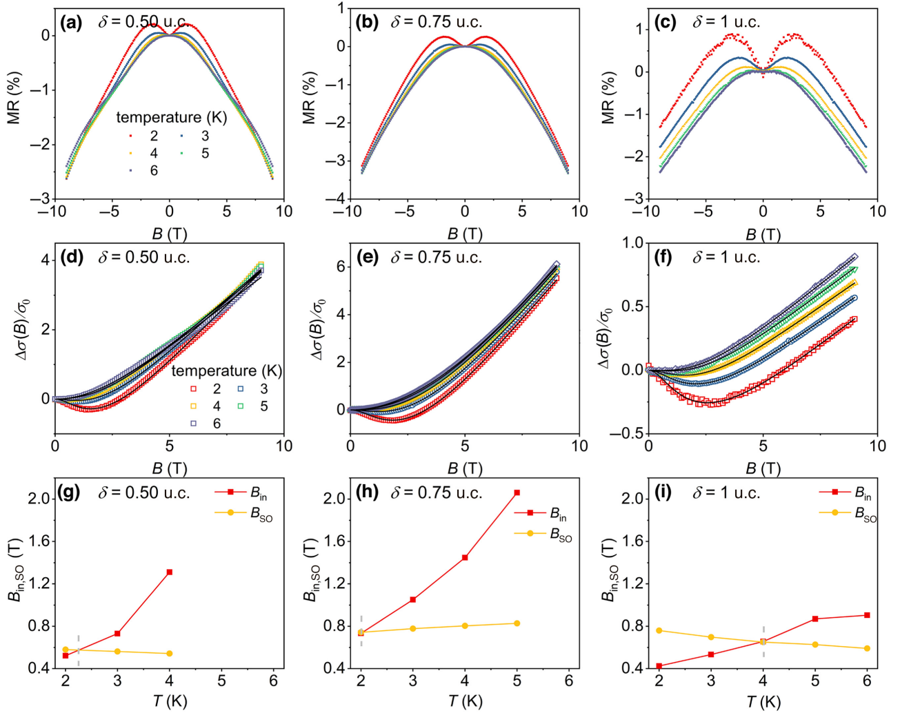
FIG. 5. (a)–(c) In-plane MR_{||} as a function of magnetic field in the low-temperature regime and sample coverages of \delta = 0.5, 0.75 , and 1 u.c., respectively. (d)–(f) \Delta\sigma/\sigma_0 values as a function of magnetic field for coverages of \delta = 0.5, 0.75 , and 1 u.c., respectively, shown as open symbols. Black solid lines are the fits obtained using Eq. (3). (g)–(i) Temperature dependence of characteristic magnetic fields ( B_{in} , B_{SO} ) for coverages of \delta = 0.5, 0.75 , and 1 u.c., respectively.
