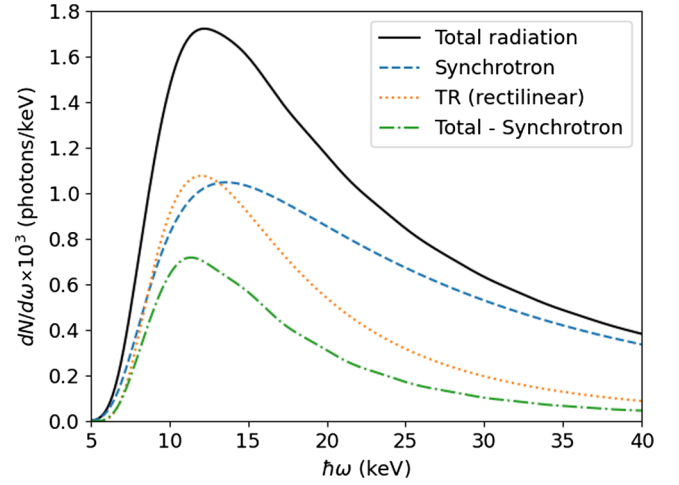
FIG. 6. Radiation spectra for the circular particle trajectory. Electron energy is 6 GeV, detector acceptance angle is 1 mrad, target thickness is 12 \mu\text{m} , electron deflection angle is \chi = 22/\gamma , and trajectory curvature radius is 13.34 m.
