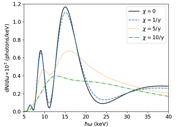
FIG. 3. Radiation spectra for the case shown in Fig. 2 for different particle deflection angles.
