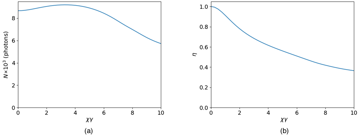
FIG. 4. Major overall characteristics of the emission for the case shown in Fig. 2. (a) Total number of photons registered by the detector and (b) ratio \eta = N/(N_{\text{TR}} + N_B) characterizing the interference effects.
