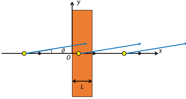
FIG. 1. Passage of a particle through a target in vacuum.
