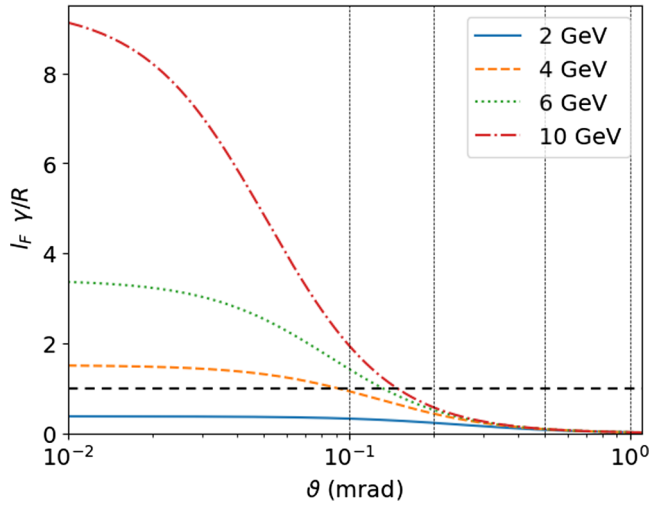
FIG. 9. Dependence of the deflection angle (in units of 1/\gamma ) within the formation length on the observation angle \vartheta for the frequency \omega = 14 keV and different electron energies. The horizontal dashed line marks the value l_F \gamma / R = 1 . The vertical lines mark the angles corresponding to the detector acceptance angles in Fig. 8 as \vartheta = \theta_0/2 .
