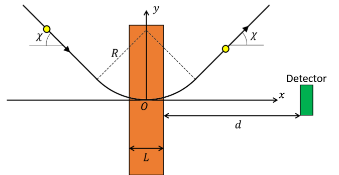
FIG. 5. Considered electron trajectory. Here \chi is the deflection angle on each side of the target, L is the thickness of the target, d is the distance between the target and the detector, and R is the curvature radius of the trajectory.
