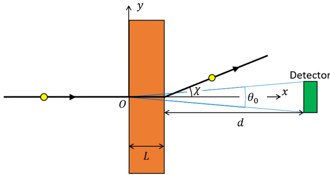
FIG. 2. Anglelike trajectory. \chi is the electron deflection angle, L is the target thickness, and d is the distance between the target and the detector.
