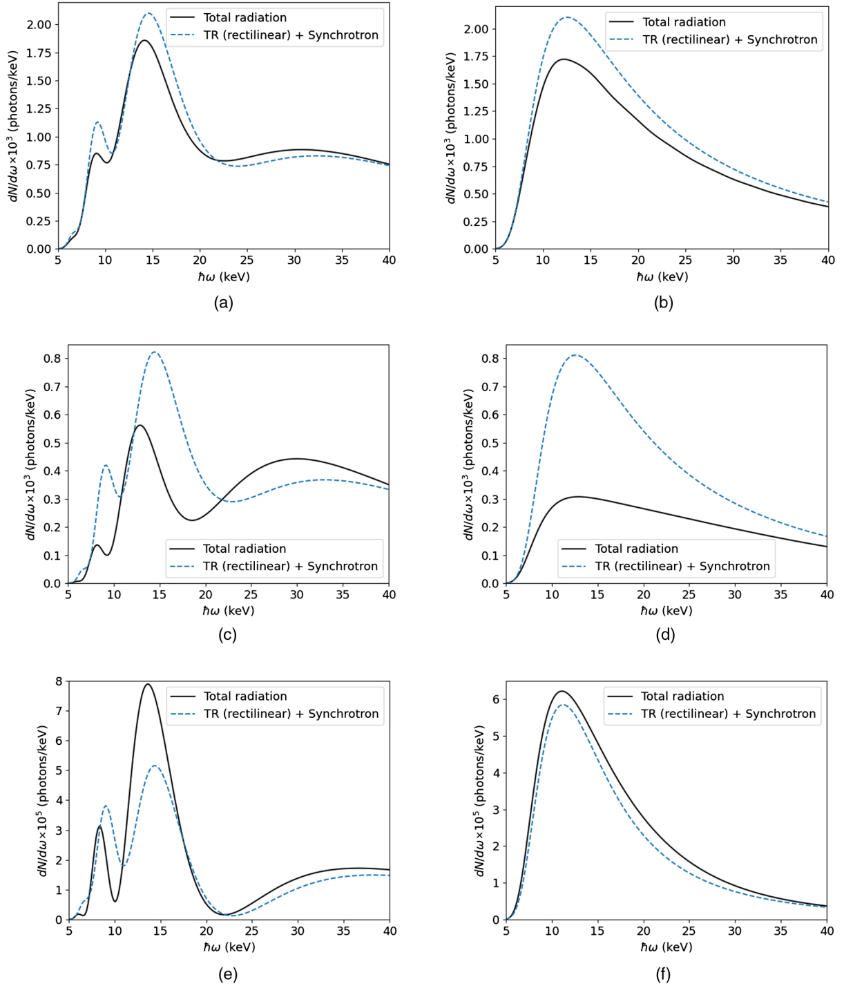
FIG. 7. Total radiation spectrum and the sum of independent spectra of TR (for a rectilinear trajectory) and SR for different target thicknesses, electron energies, and detector acceptance angles: (a) 6 GeV, 1 mrad, 50 \mu\text{m} ; (b) 6 GeV, 1 mrad, 12 \mu\text{m} ; (c) 6 GeV, 0.4 mrad, 50 \mu\text{m} ; (d) 6 GeV, 0.4 mrad, 12 \mu\text{m} ; (e) 2 GeV, 0.4 mrad, 50 \mu\text{m} ; and (f) 2 GeV, 0.4 mrad, 12 \mu\text{m} .
