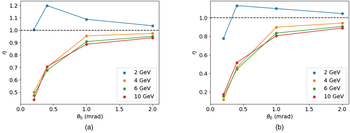
FIG. 8. Dependence of the ratio \eta = N/(N_{\text{TR}} + N_{\text{SR}}) on the acceptance angle \theta_0 . (a) Target thickness is 50 \mu\text{m} and (b) target thickness is 12 \mu\text{m} .
