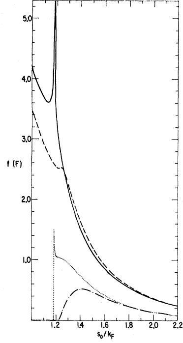
FIG. 12. Real and imaginary parts of independent-pair scattering amplitudes calculated for the Wheeler-Yamaguchi (Refs. 7, 8) potential with the parameters \lambda = 0.425 \text{ F}^{-3} , \beta = 1.46 \text{ F}^{-1} , and k_F = 1.42 \text{ F}^{-1} . The calculations were performed using Eqs. (8), (15), and (16) in the text. The solid and dotted lines represent the real and imaginary parts, respectively, of the scattering amplitude obtained for (k_{10}/k_F) = 1.2 , (k_{20}/k_F) = 0.9 , and \cos\theta = 1.0 . The dashed and dot-dashed lines show the real and imaginary parts, respectively, of the scattering amplitude obtained for (k_{10}/k_F) = 1.2 , (k_{20}/k_F) = 0.7 , and \cos\theta = 1.0 .
