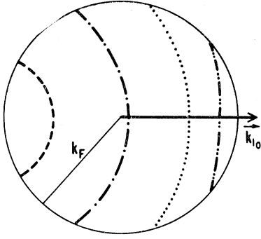
FIG. 4. A schematic illustration of sets of particles within the Fermi sphere which, when paired with an incident particle having the wave vector k_{i0} , lead to center-of-mass wave vectors \Lambda_0 of equal magnitude. The solid circle indicates the Fermi sphere. The dashed, dot-dashed, dotted, and dashed-double-dotted arcs are loci of the terminating points of wave vectors which lead to a fixed value of \Lambda_0 . The value of \Lambda_0 associated with these arcs increases monotonically as one moves from the dashed arc to the dashed-double-dotted arc.
