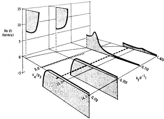
FIG. 7. The real part of the independent-pair scattering amplitude calculated for the Wheeler-Yamaguchi (Refs. 7, 8) potential with the parameters \lambda = 0.425 \text{ F}^{-3} and \beta = 1.46 \text{ F}^{-1} . The calculations were performed using Eqs. (8), (15), and (16) in the text with the kinematical parameters k_{10} = 1.562 \text{ F}^{-1} , k_{20} = 0.1775 \text{ F}^{-1} , and \cos\theta = -1.0 . The solid lines represent the real part of the scattering amplitude. The shading is included only for ease in visualization. The heavy dashed line indicates the energy-shell value, k_{10} , of s_0 . The dotted line designates the location of the bound-state pole in the scattering amplitude. The curving light line at which the graphs of \text{Re}(f) begin indicates the point s_0 = k_F for the various values of k_F . The s_0 scale is measured in units of p_F = (k_F)_{\text{obs}}/8 .
