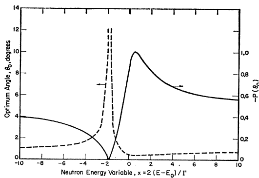
FIG. 2. The optimum angle for polarization \theta_0 and the polarization P(\theta_0) as a function of energy near a "pure" s -wave resonance ( \rho=0 ) for kR=0.5 .
