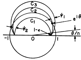
FIG. 1. Circular arcs C_1 , C_2 , and C_3 .
