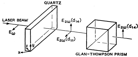
FIG. 1. Schematic drawing showing the orientation of the quartz sample with respect to the polarized laser beam for separating the second harmonic light waves due to the two nonlinear coefficients d_{11} and d_{14} .
