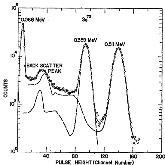
FIG. 1. Singles \gamma -ray spectrum of the decay of \text{Se}^{73} as viewed by a 3-in. \times 3-in. NaI(Tl) detector. Individual \gamma -ray contributions are represented by dashed lines.
