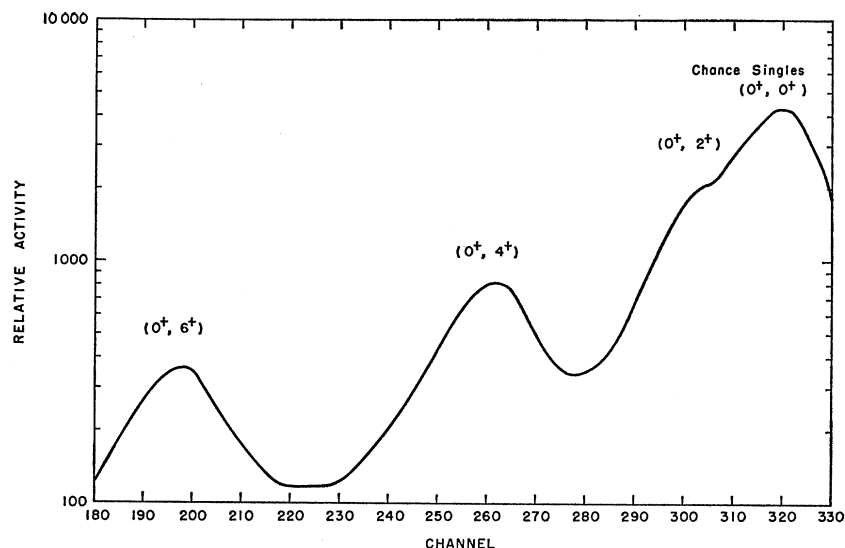
FIG. 2. Gamma-alpha coincidence spectrum of \text{Cf}^{246} .
