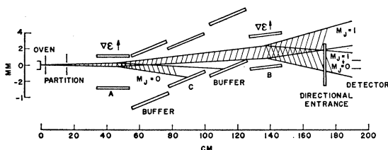
FIG. 3. Schematic view of the apparatus.
