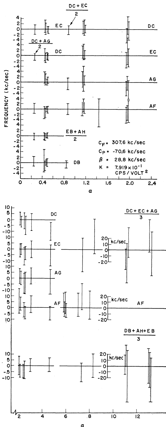
FIG. 6. All HF data plotted relative to the lines calculated by using the adopted values of the hfs constants and K_{\text{HF}} . Each point consists of two frequency scans in opposing directions.
