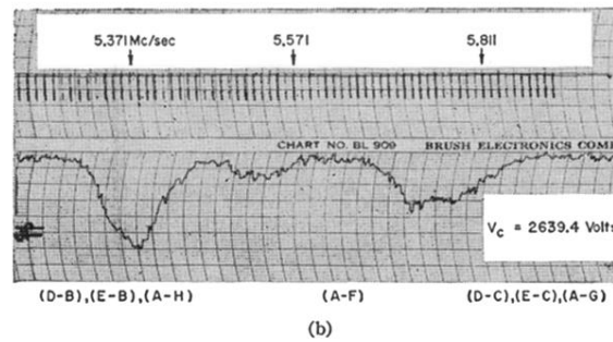
FIG. 5. (a) HF spectrum at C -field voltage of 748.10 V, which corresponds to \alpha=0.4803 . Lock-in detector time constant, 5 sec. Down indicates increasing beam intensity. Frequency markers are 10 kc/sec apart. (b) HF spectrum at C -field voltage of 2639.4 V, which corresponds to \alpha=5.978 . Lock-in detector time constant, 1 sec.
