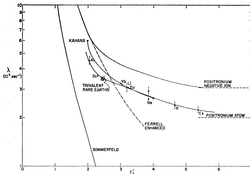
FIG. 4. Annihilation rate vs r_s' for Al and the metals of groups I A and III B. The annihilation rates for the alkali metals were taken from the work of Bell and Jorgensen (reference 3) and adjusted slightly as described in the text. The lower of the two points labeled Na is from the present investigation. A smooth curve is drawn through the experimental points, and various theoretical curves are shown for comparison.
