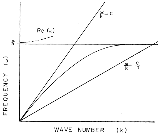
FIG. 1. Shape of the dispersion curve for electron plasma oscillations along a plasma slab or cylinder in a strong magnetic field ( B_0 \parallel \mathbf{k} ).
