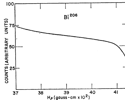
FIG. 15. Calculated positron spectrum of \text{Bi}^{206} with 0.25% \text{Bi}^{205} contamination.
